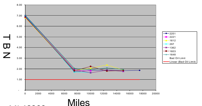
Raw Chart - TBN vs. Mileage
