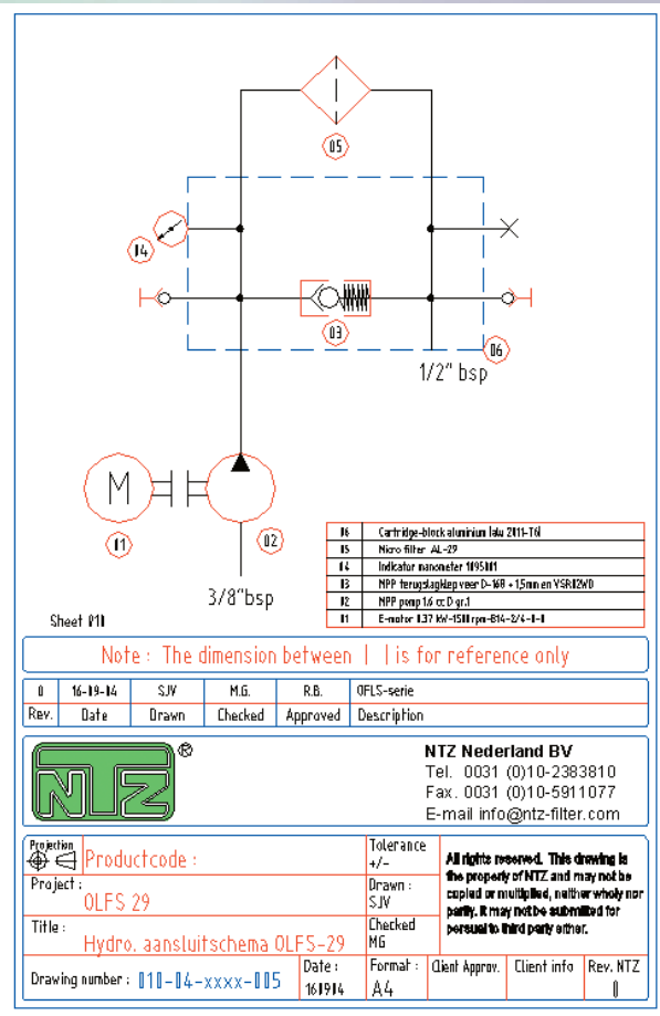
Hydraulic Scheme OLFS
